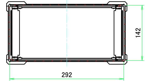
C-C (1:5)
