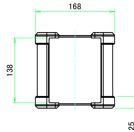
C view
