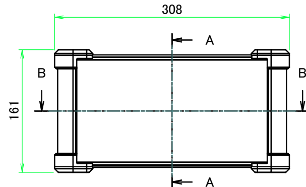
A view
