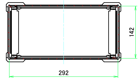
C-C (1:5)
