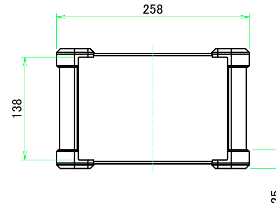
C view
