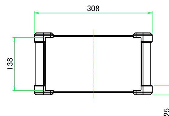
C view
