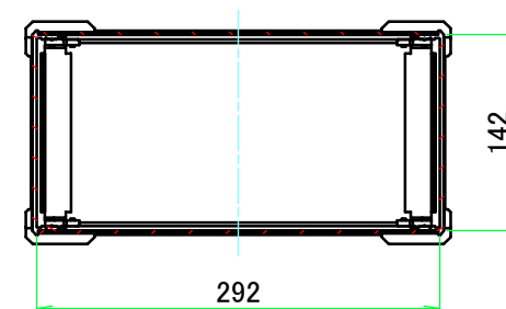
C-C (1:6)
