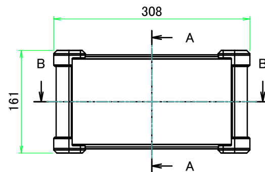
A view
