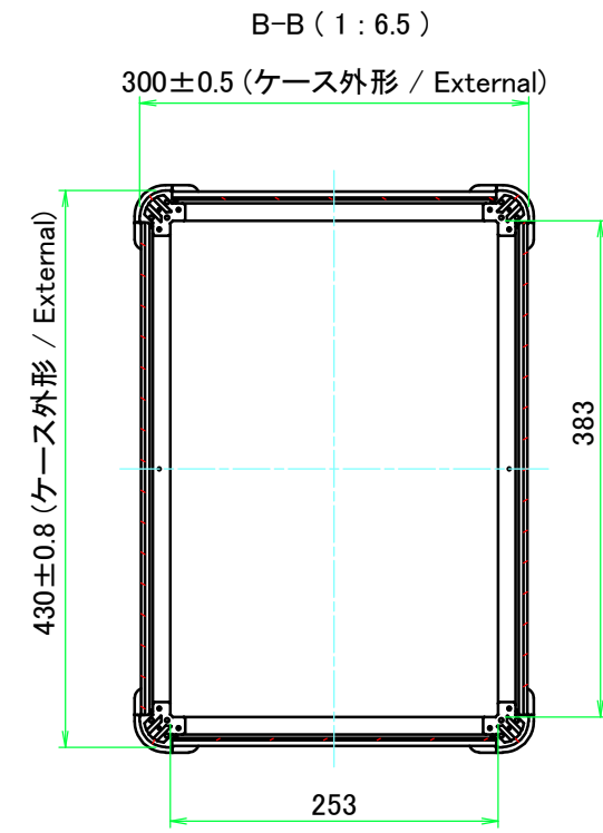
D view
