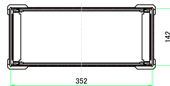
C-C (1:5.5)
