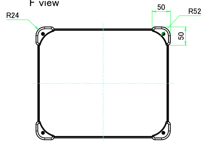
F view
