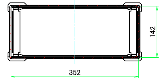
C-C (1:6)
