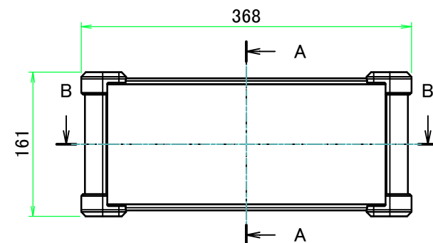
A view
