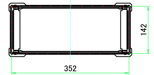
C-C (1:7)
