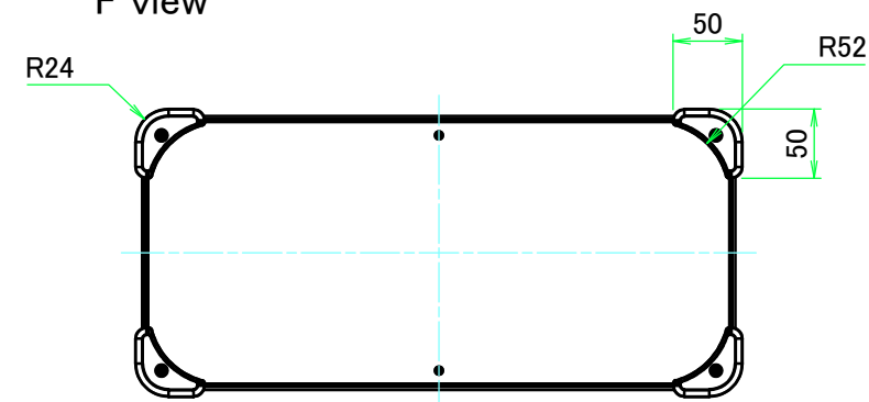
F view
