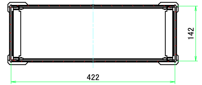
C-C (1:6)
