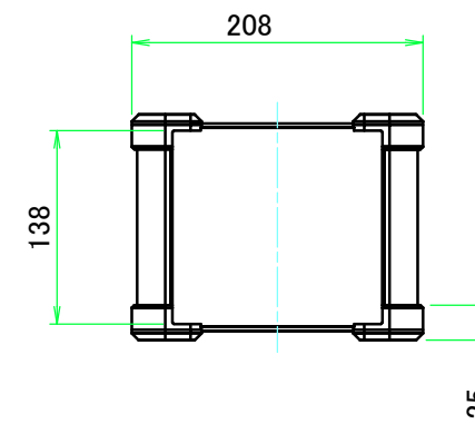
C view
