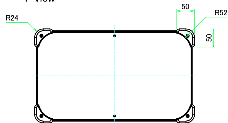
F view
