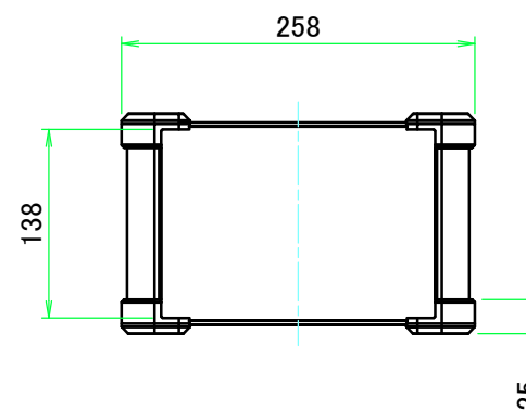
C view
