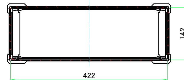
C-C (1:6)
