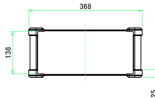
C view
