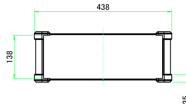
C view
