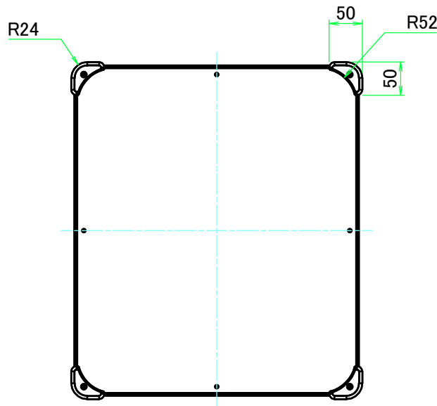
F view
