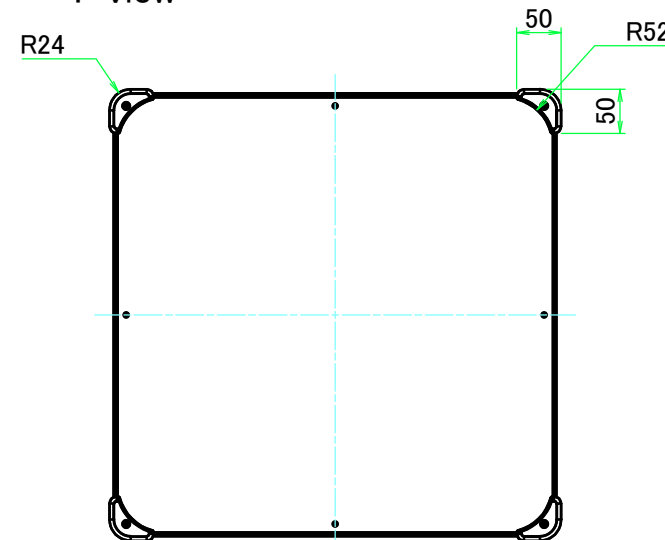
F view
