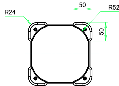
F view
