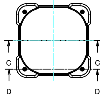
E view
