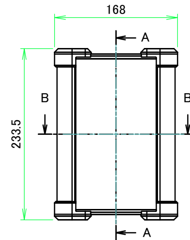
A view
