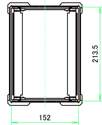
C-C (1:5)
