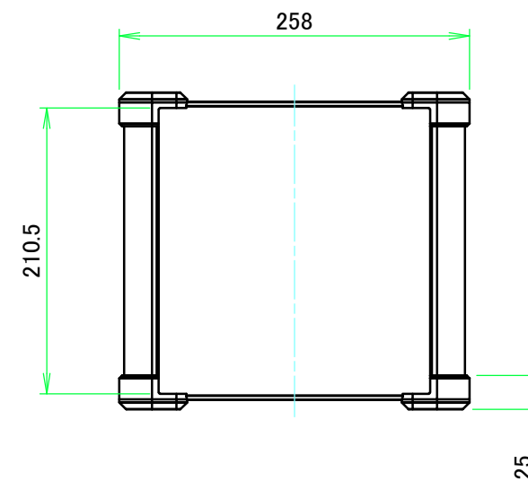
C view
