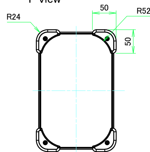
F view
