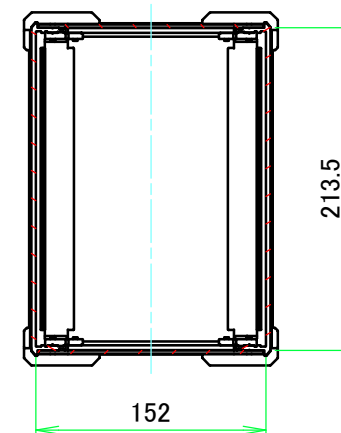
C-C (1:5)
