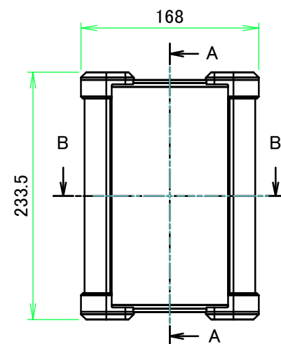
A view
