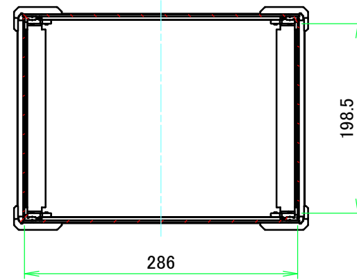
A-A (1:5.5)
