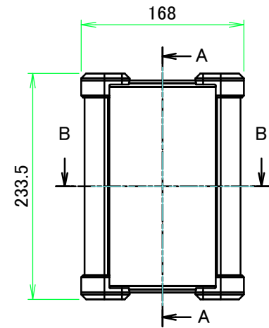
A view
