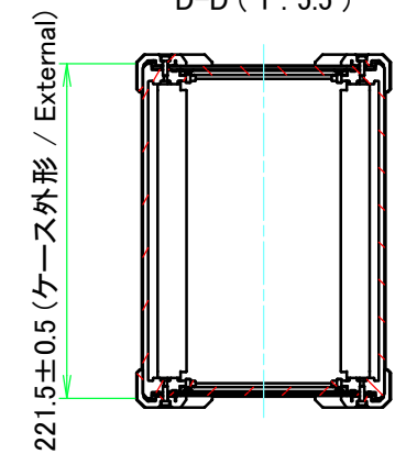
D-D (1:5.5)
