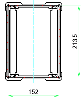
C-C (1:5.5)
