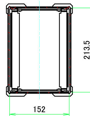
C-C (1:6)
