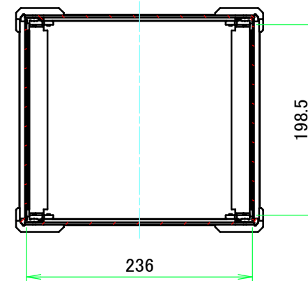
A-A (1:5.5)
