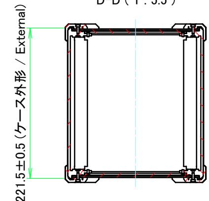
D-D (1:5.5)
