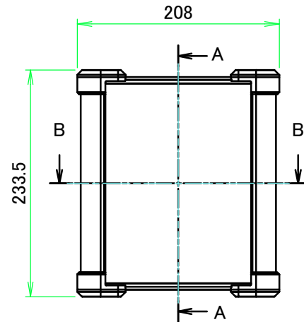
A view
