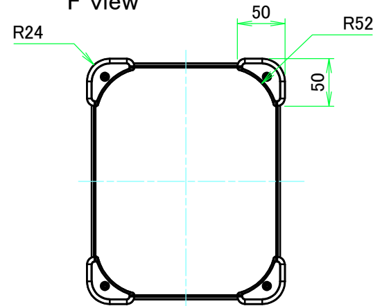
F view
