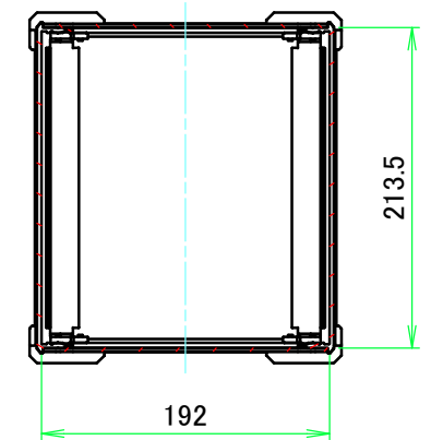
C-C (1:5.5)
