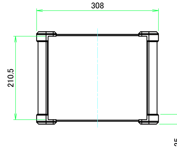
C view
