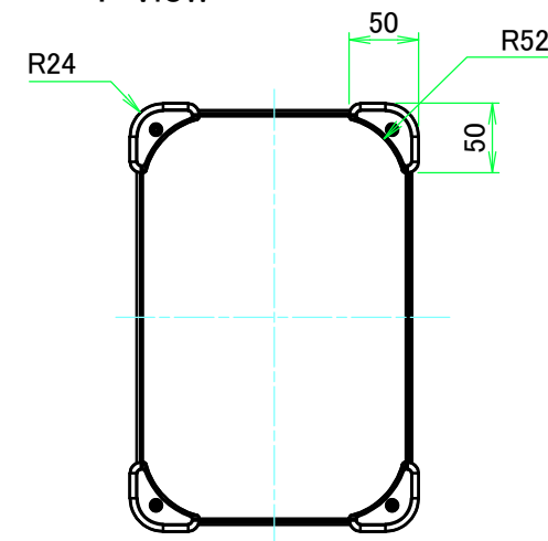
F view
