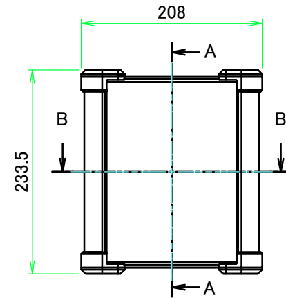
A view
