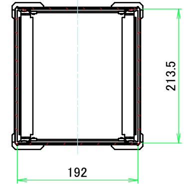
C-C (1:6)
