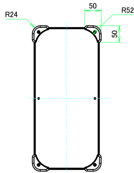
F view
