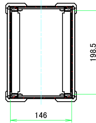
A-A (1:5.5)
