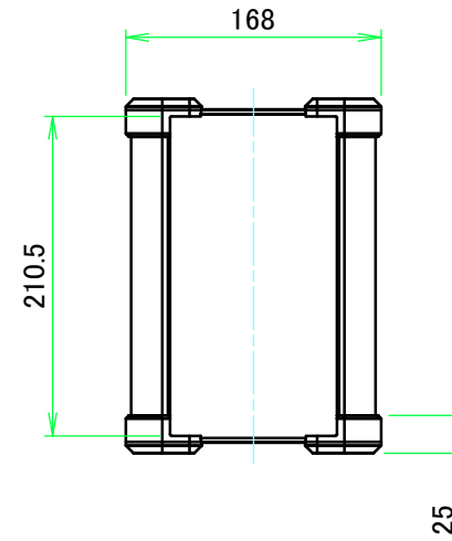
C view
