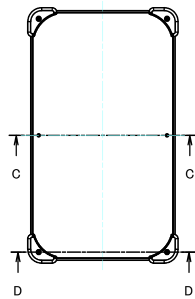
A view
