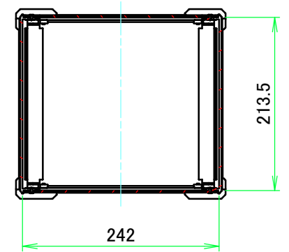
C-C (1:6.5)
