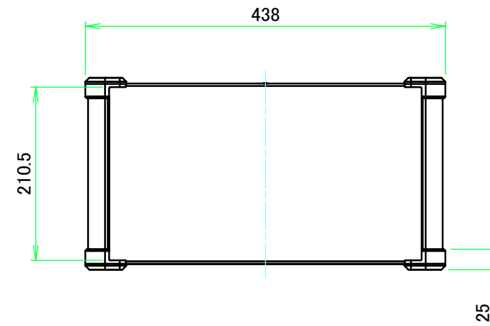
C view
