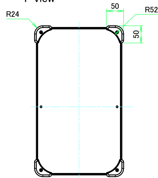
F view
