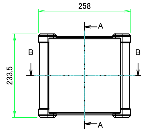
A view
