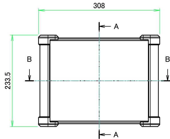
A view
