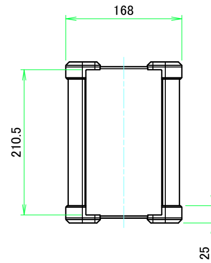
C view
