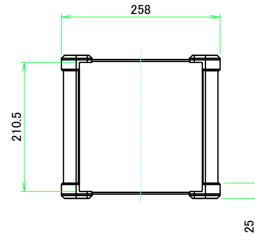
C view
