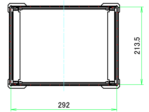
C-C (1:6)
