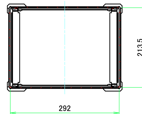
C-C (1:6)
