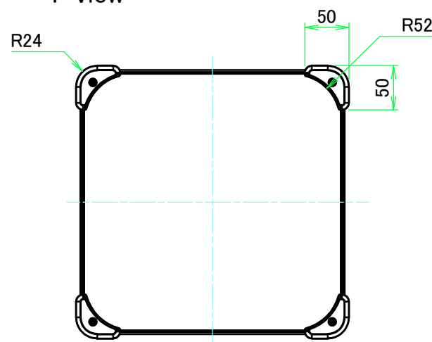
F view
