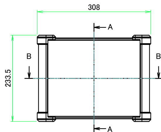
A view
