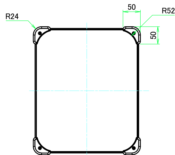
F view
