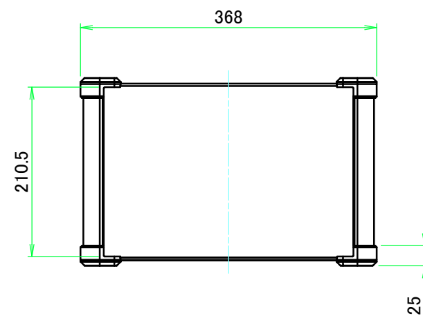
C view
