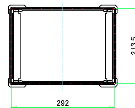
C-C (1:6.5)
