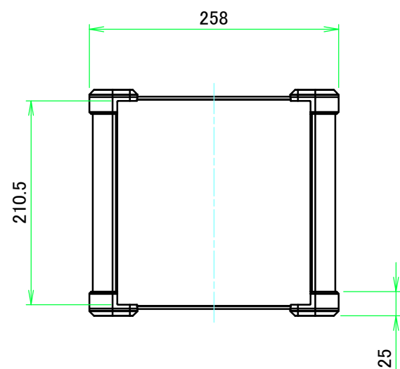
C view
