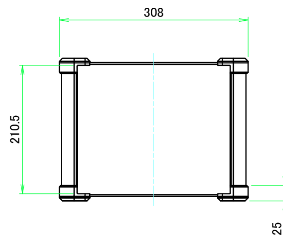
C view
