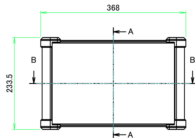
A view
