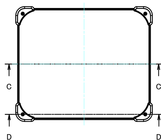
E view
