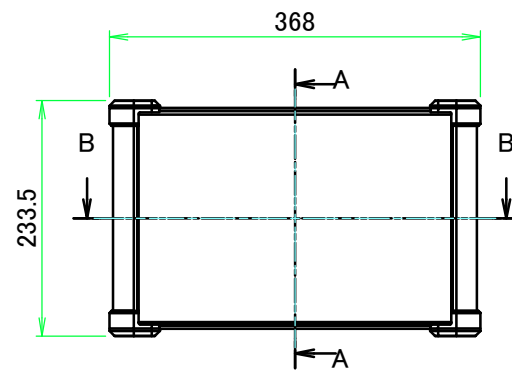
A view
