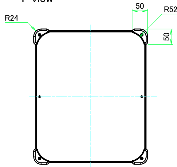
F view
