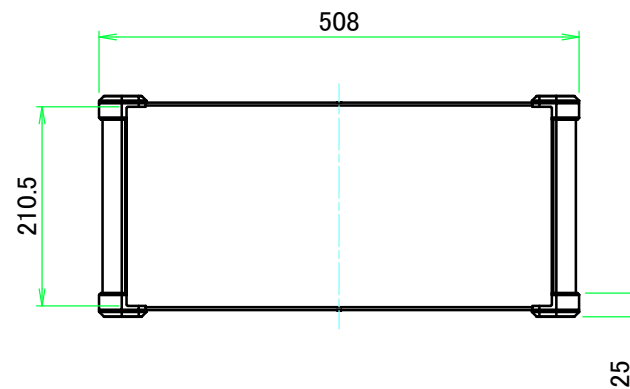
C view
