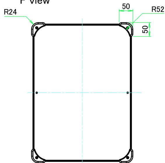
F view
