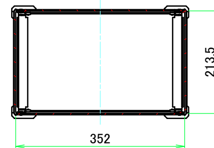
C-C (1:8)
