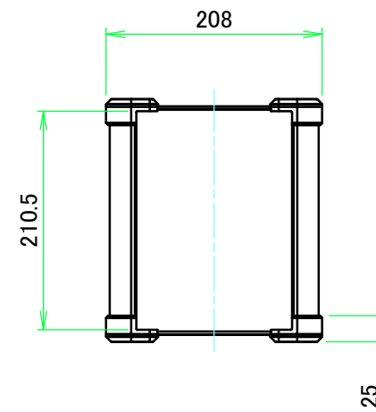
C view
