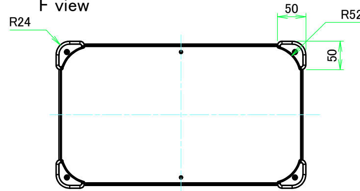
F view
