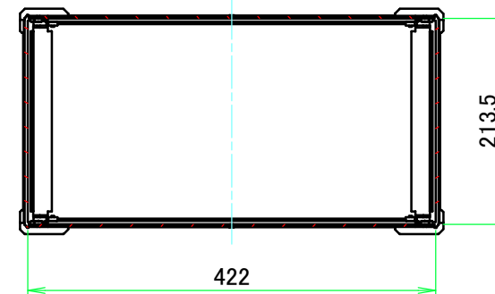
C-C (1:7)
