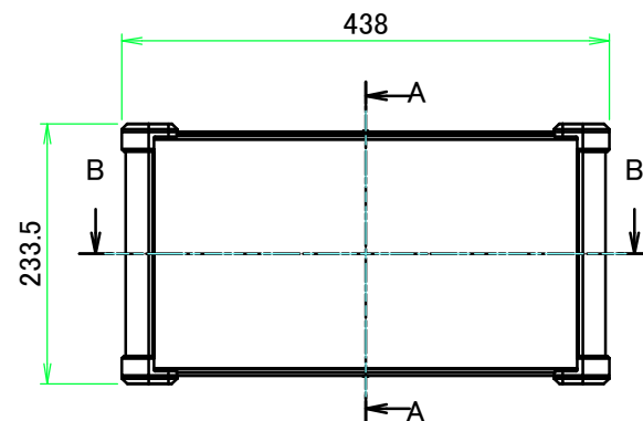
A view
