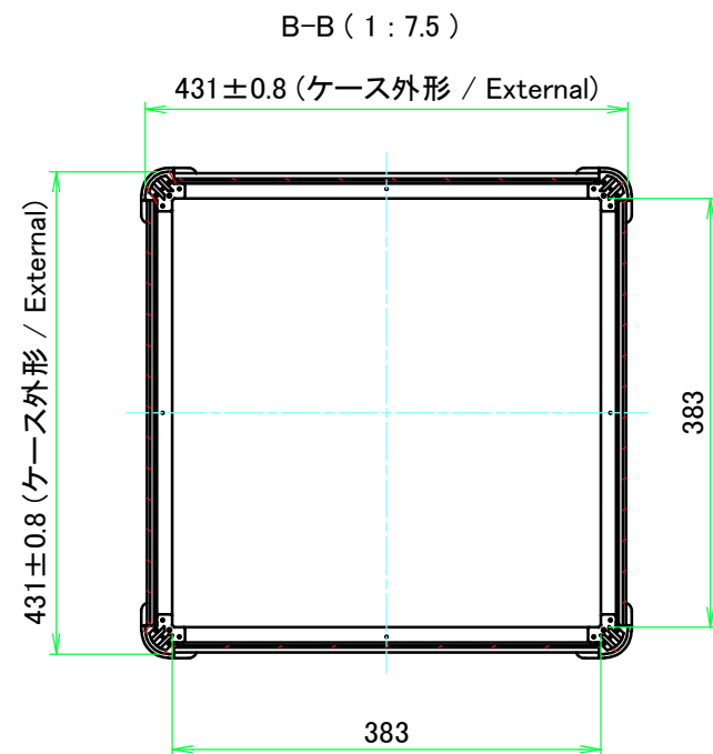
D view
