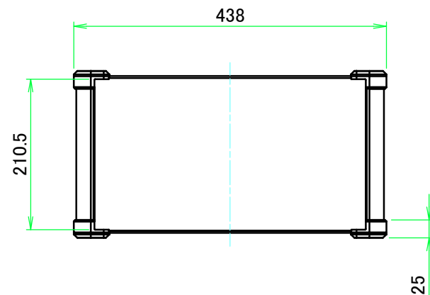
C view
