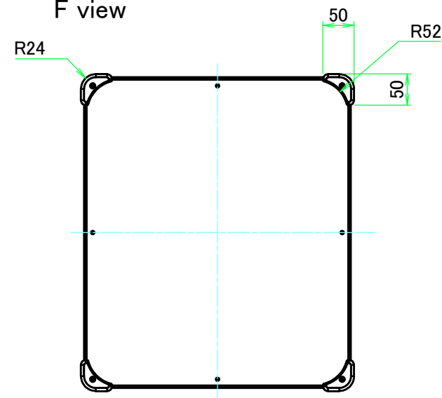
F view
