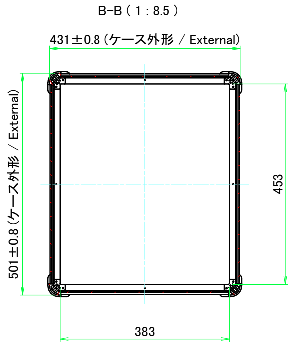
D view
