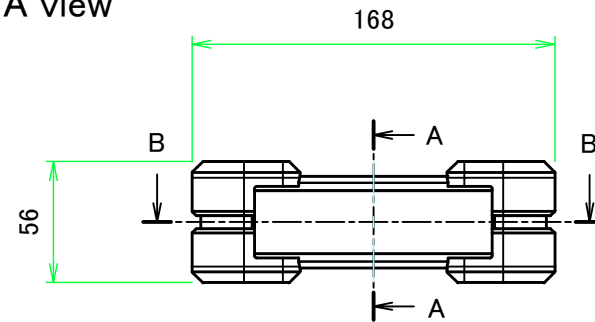
A view
