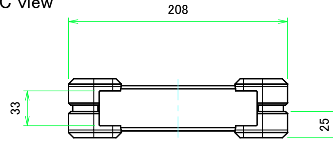
C view
