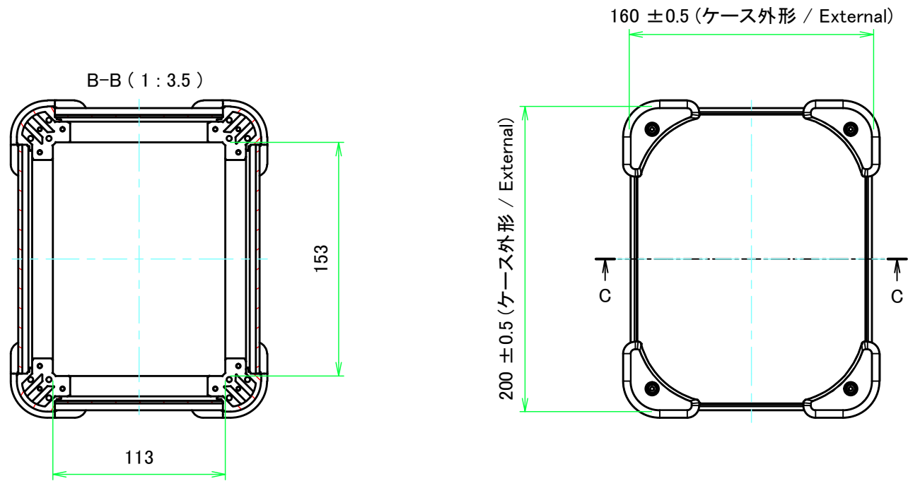
E view
