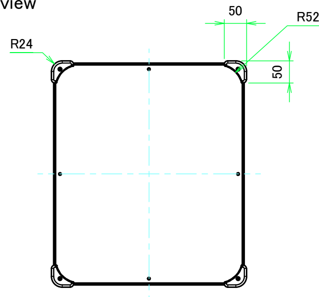
F view
