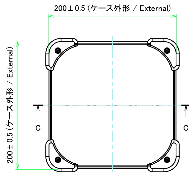
E view
