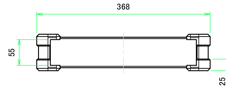
C view
