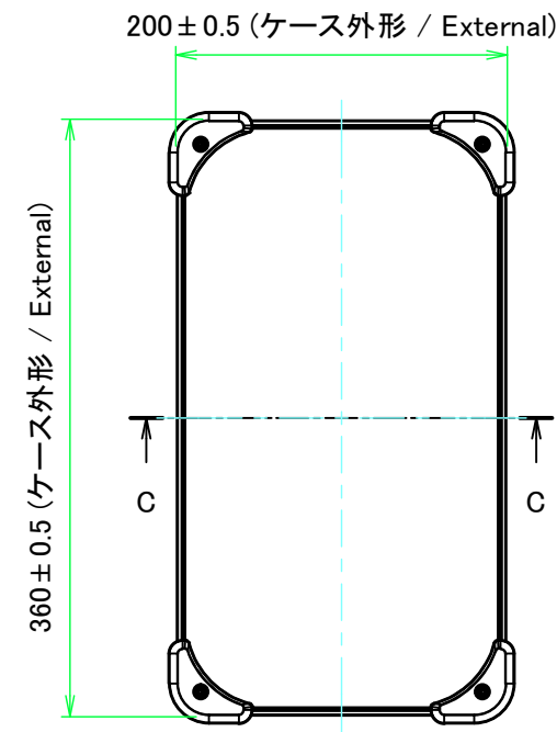
E view
