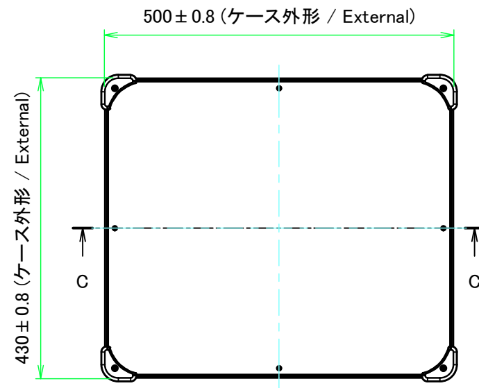
E view
