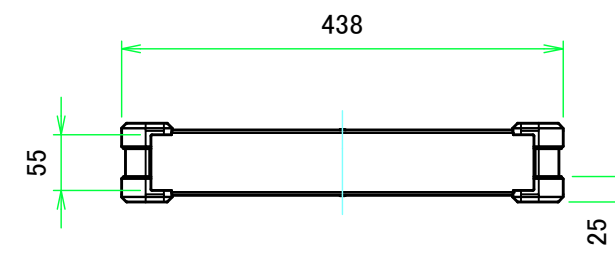
C view
