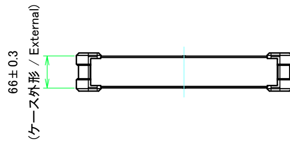
D view
