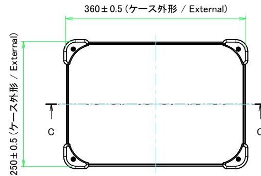
E view
