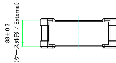
D view
