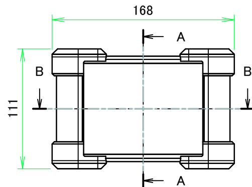
A view
