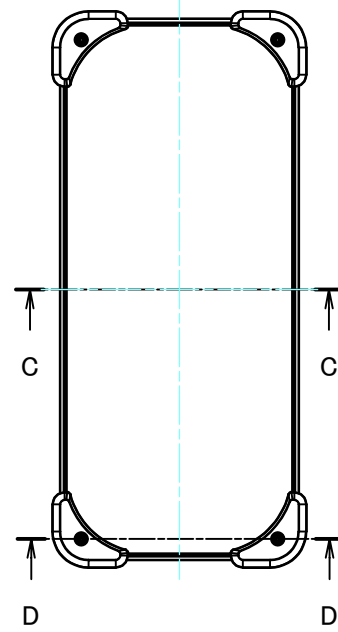
E view
