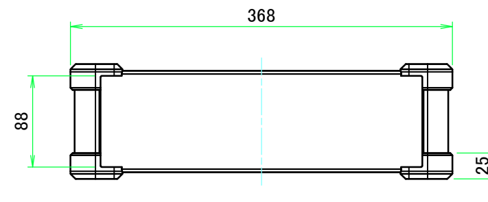
C view
