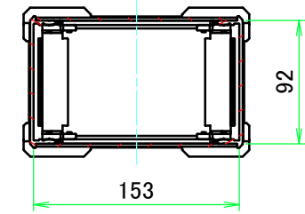
C-C (1:5)
