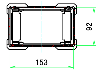
C-C (1:5.5)
