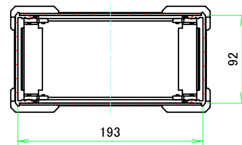
C-C (1:4)
