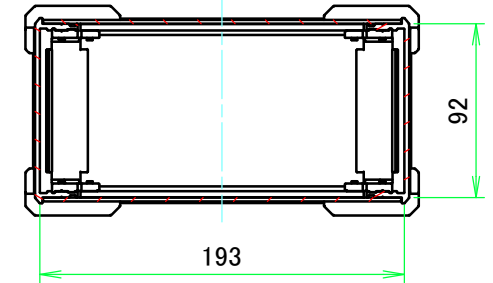
C-C (1:4)
