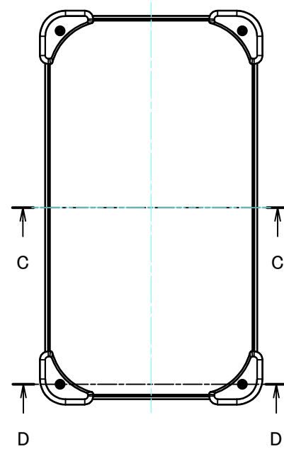
E view
