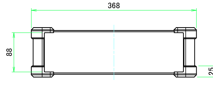
C view
