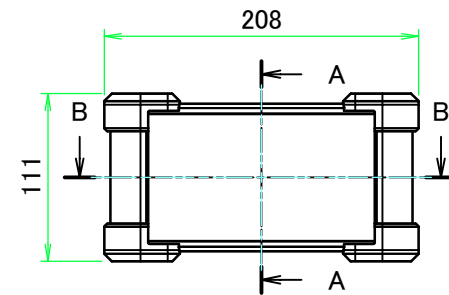
A view
