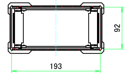
C-C (1:5)
