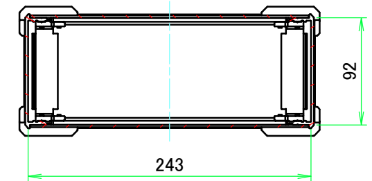
C-C (1:4.5)
