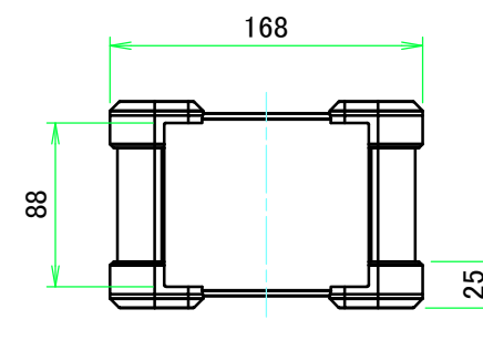
C view
